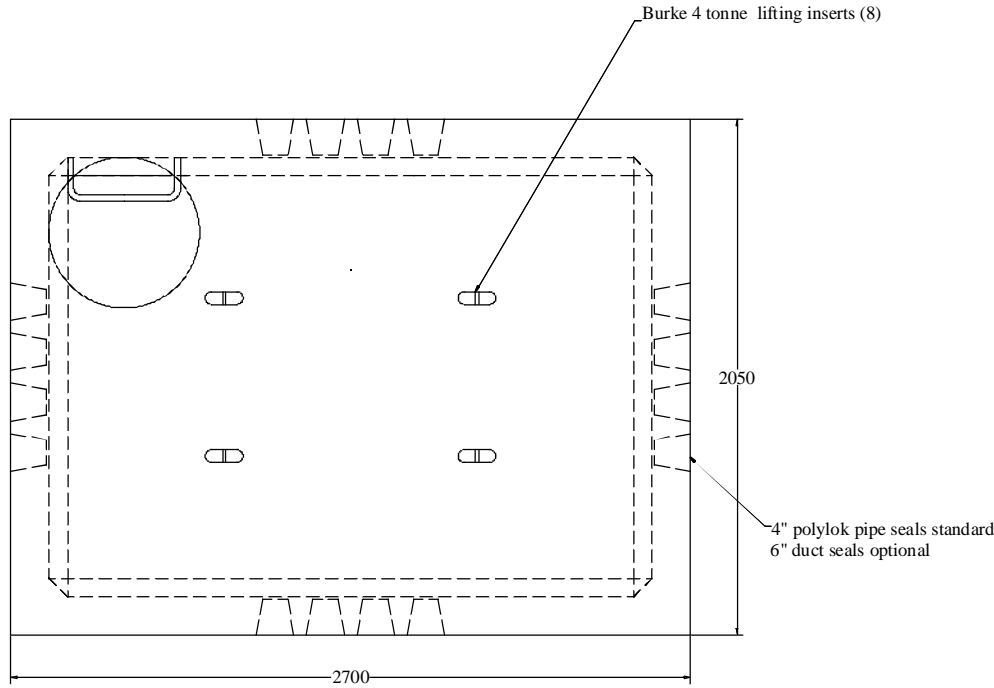
Top View
